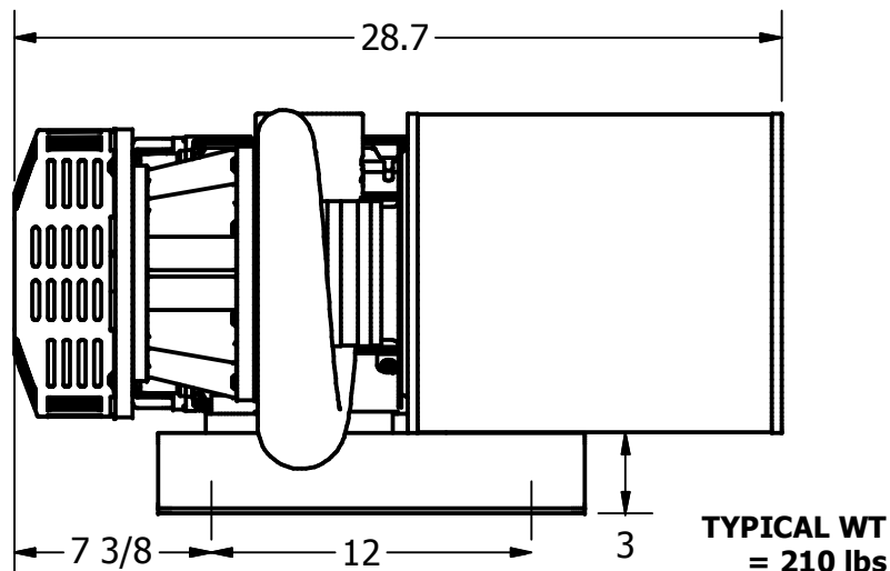
8008256 FILTER / SILENCER
