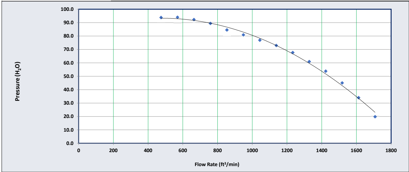
Motor / Blower pulley ratio @ 60Hz
